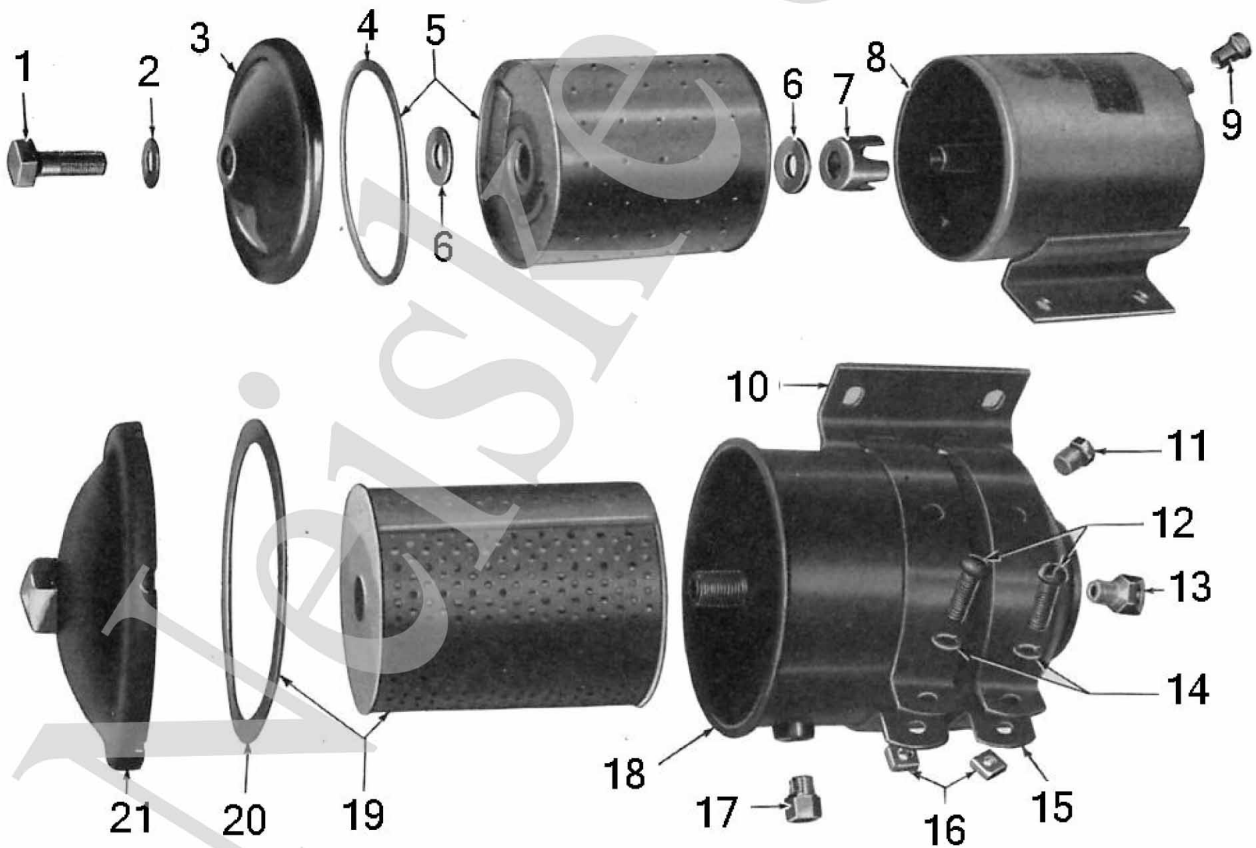
Ölfilter / Oil filter
