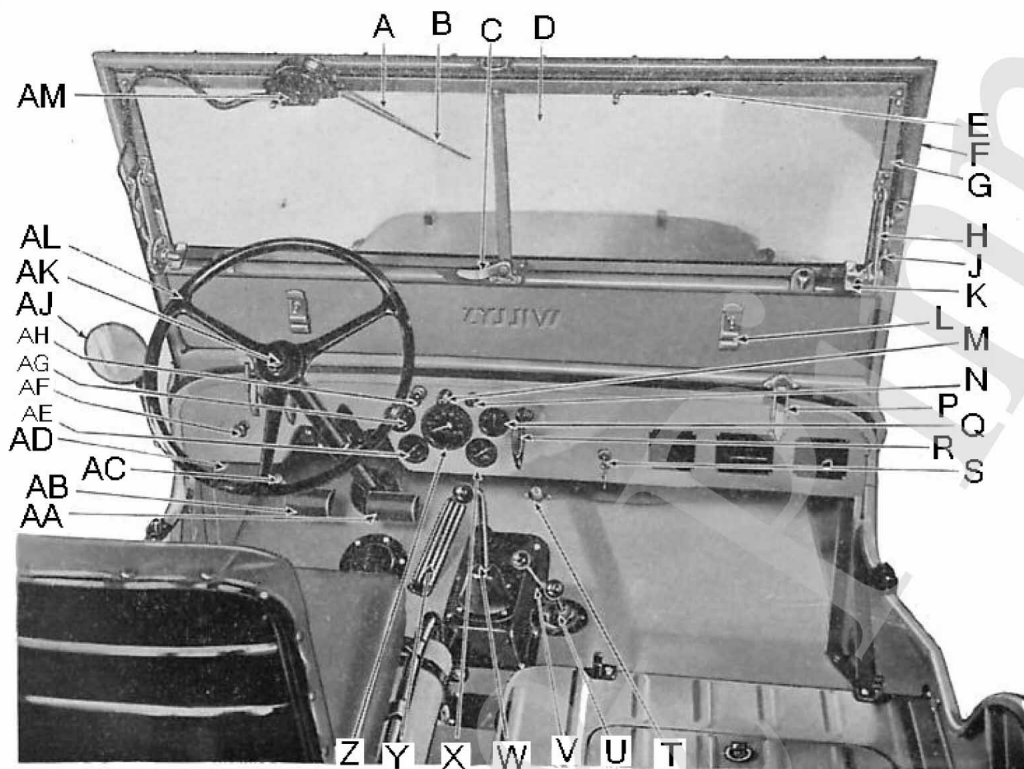
Armaturenbrett / Front compartment CJ 2A
