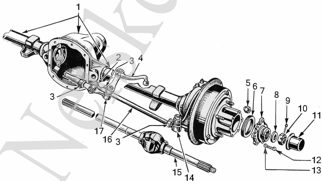
Vorderachse / Front axle
