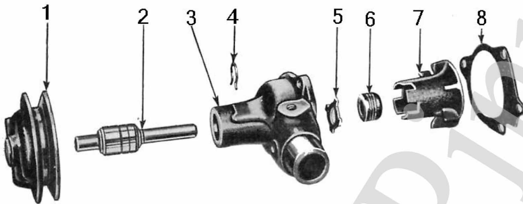
Wasserpumpe / Water pump
