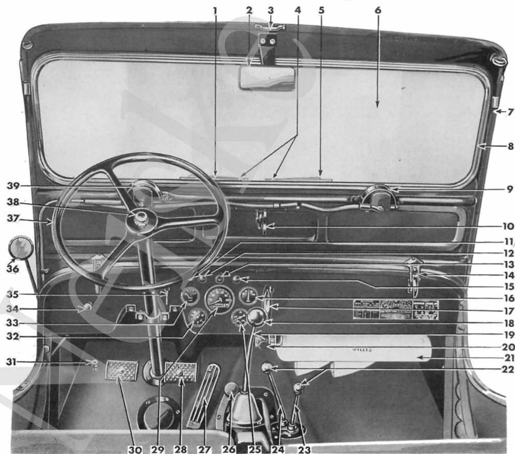
Armaturenbrett / Front compartment CJ 3A
