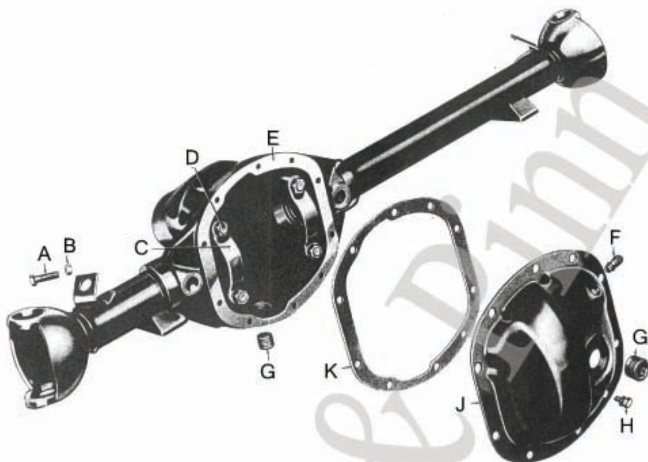
Vorderachse / Front axle
