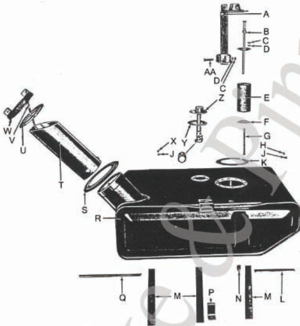
Tank / Fuel tank
