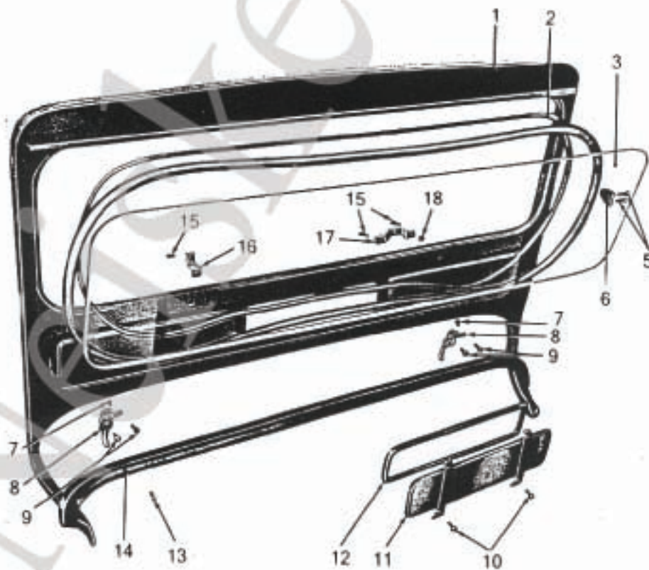
Scheibenrahmen / Windshield and related parts
