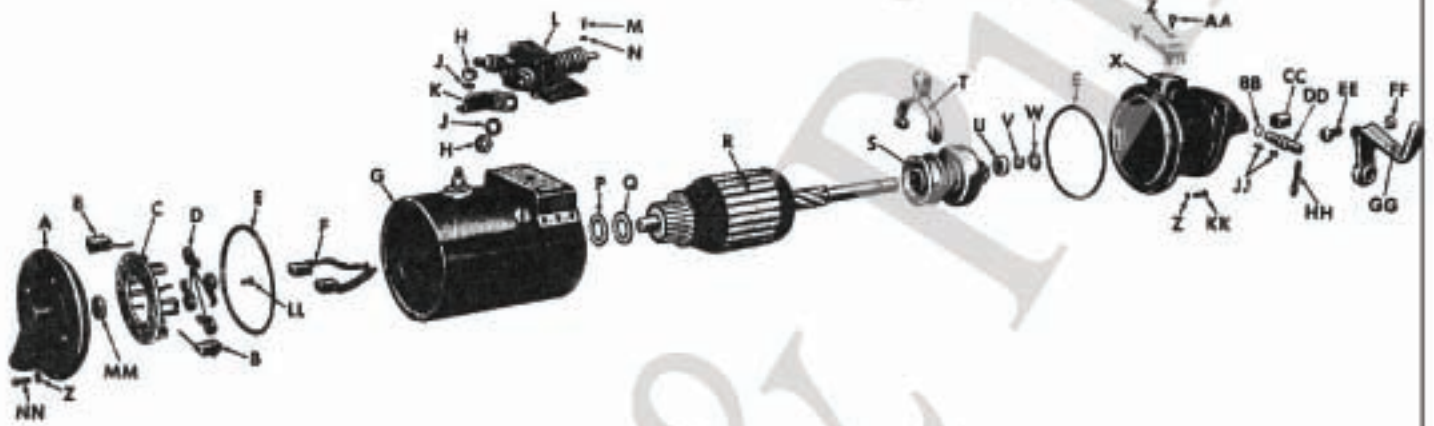
Anlasser / Starter
