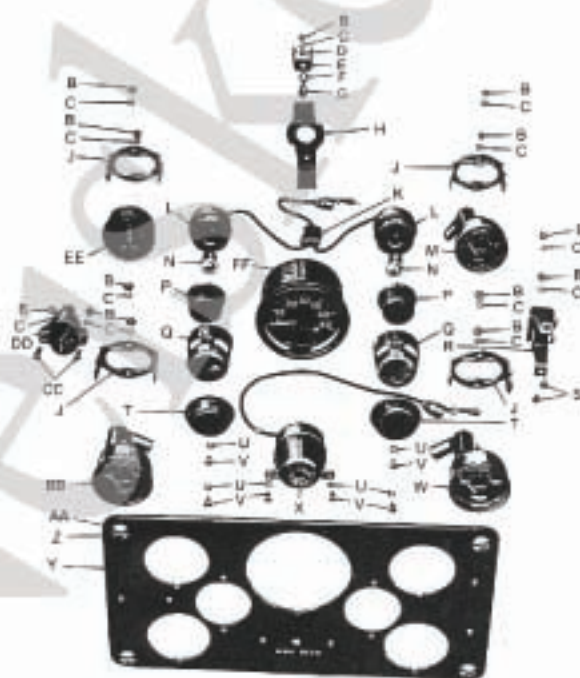
Instrumente / Instrument cluster
