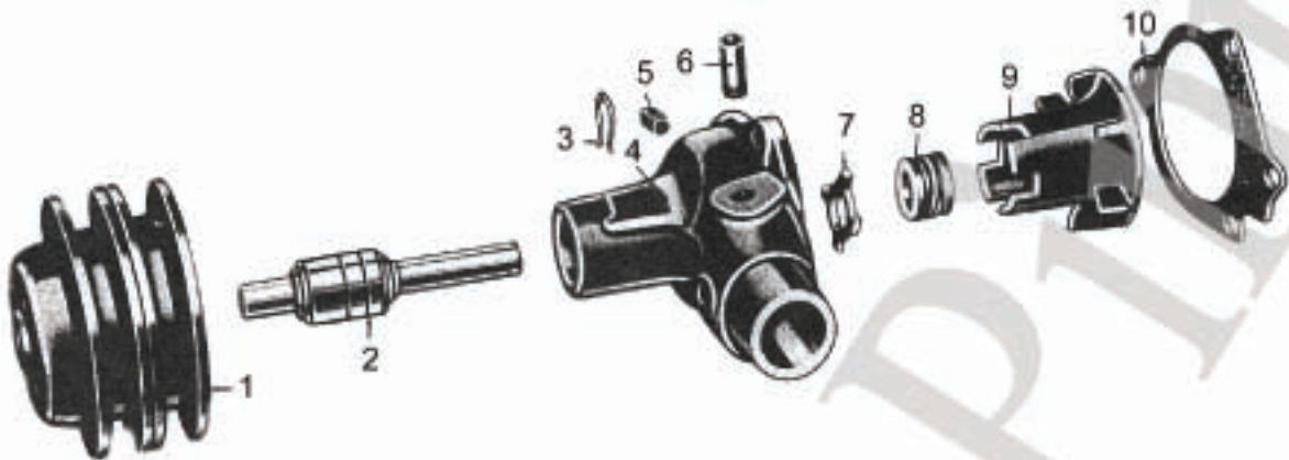
Wasserpumpe / Water pump
