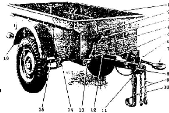
FIG. 21—FRONT VIEW OF TRAILER
