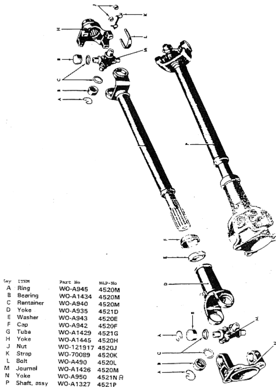
Rear propeller shaft Page 21
