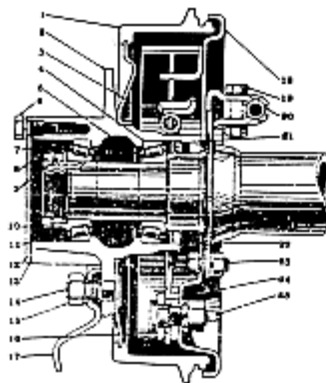
FIG. 13—WHEEL BEARING
