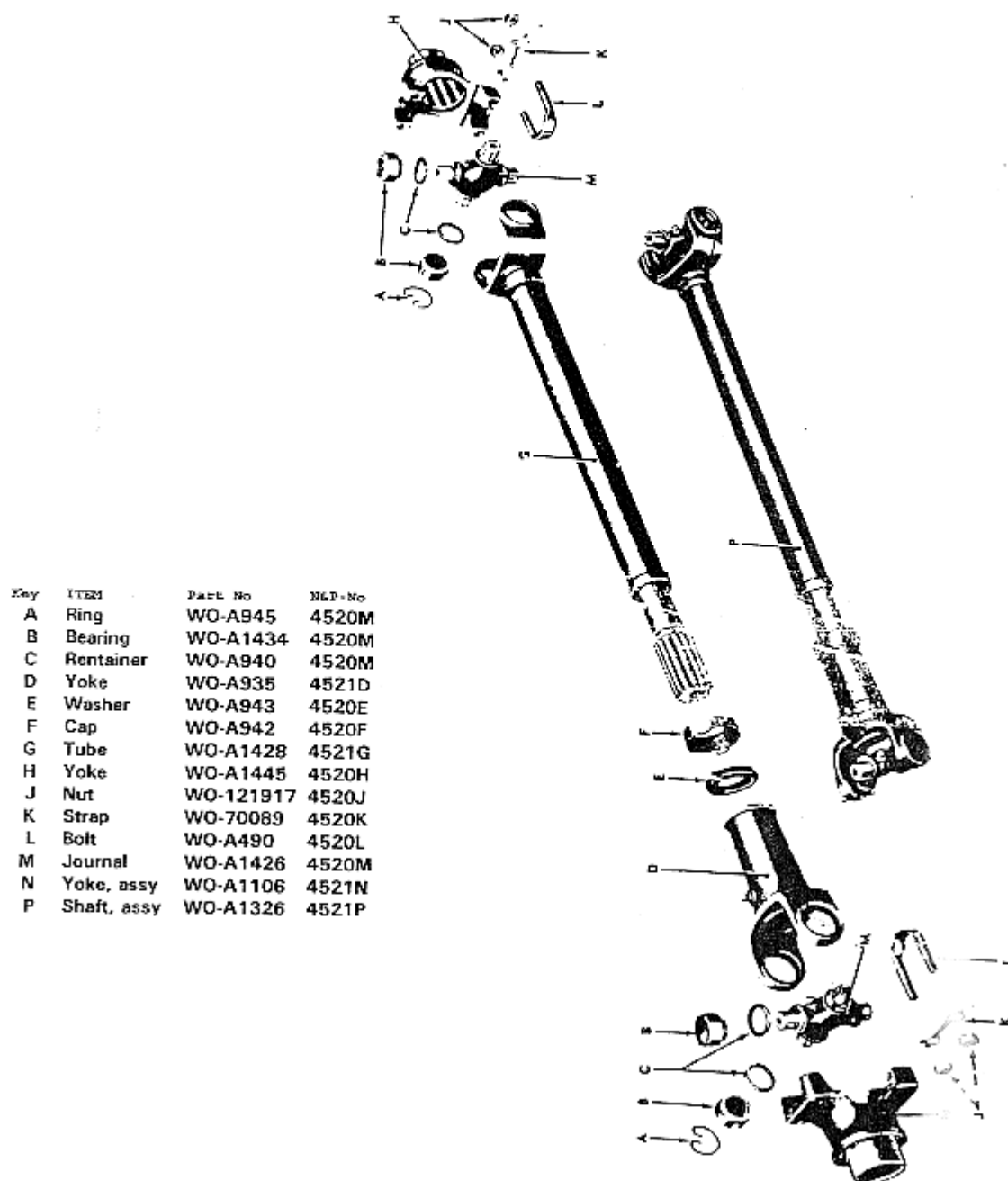
Front propeller shaft Page 20
