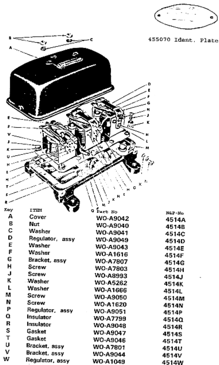
Generator regulator, 6-volt-assembly Page 14
