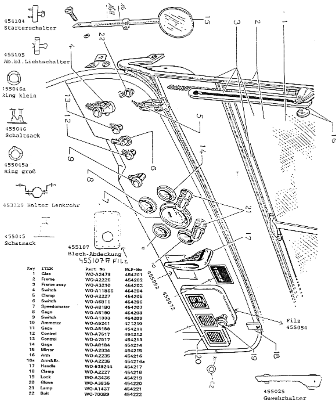
Front compartment and instrument panel Page 42
