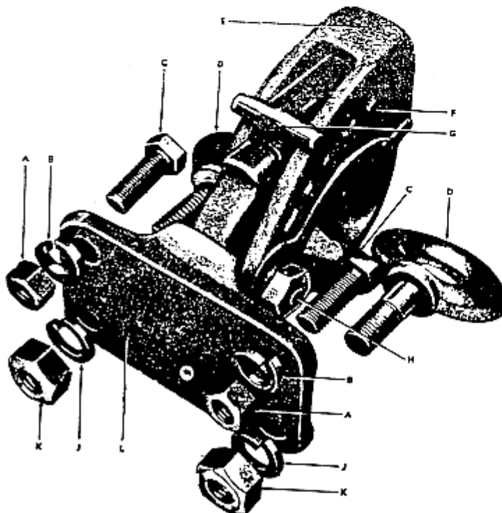
Pintel assembly Page 44
