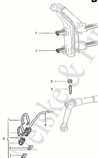
Page 26B Federstab Stabilisator
