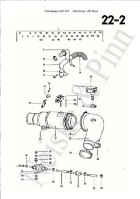
Page 22-2 Standheizung
