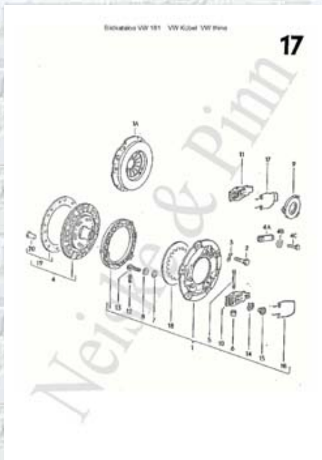
Page 17 Kupplung
